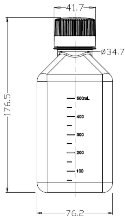
500 mL (square-shouldered model)
